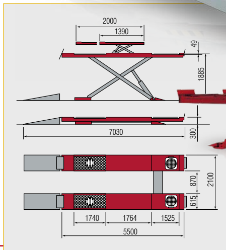
RAV 650.2.55SI - 5000 kg Assetto/Alignment
