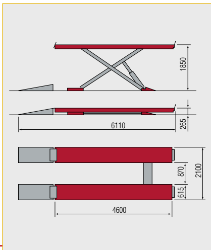
RAV 635.1 - 3500 kg Pedane piane/Flat runways
